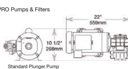
Standard Plunger Pump
