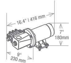
HP Pump (modular 170)
