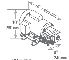
HP Pump
