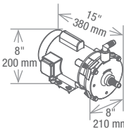
Booster Pump
