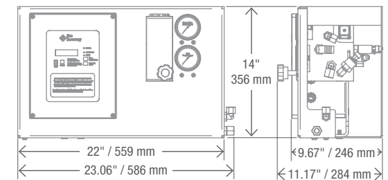
Control Panel - Front
