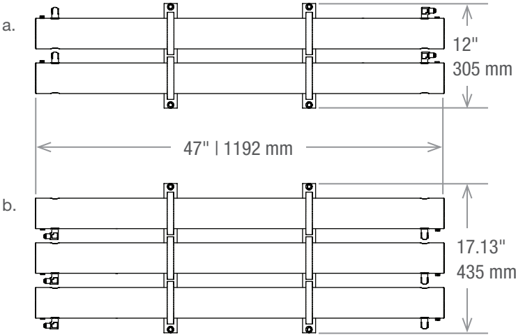
Membrane assembly (a. ZK-B2-F | b. ZK-B3-F)
